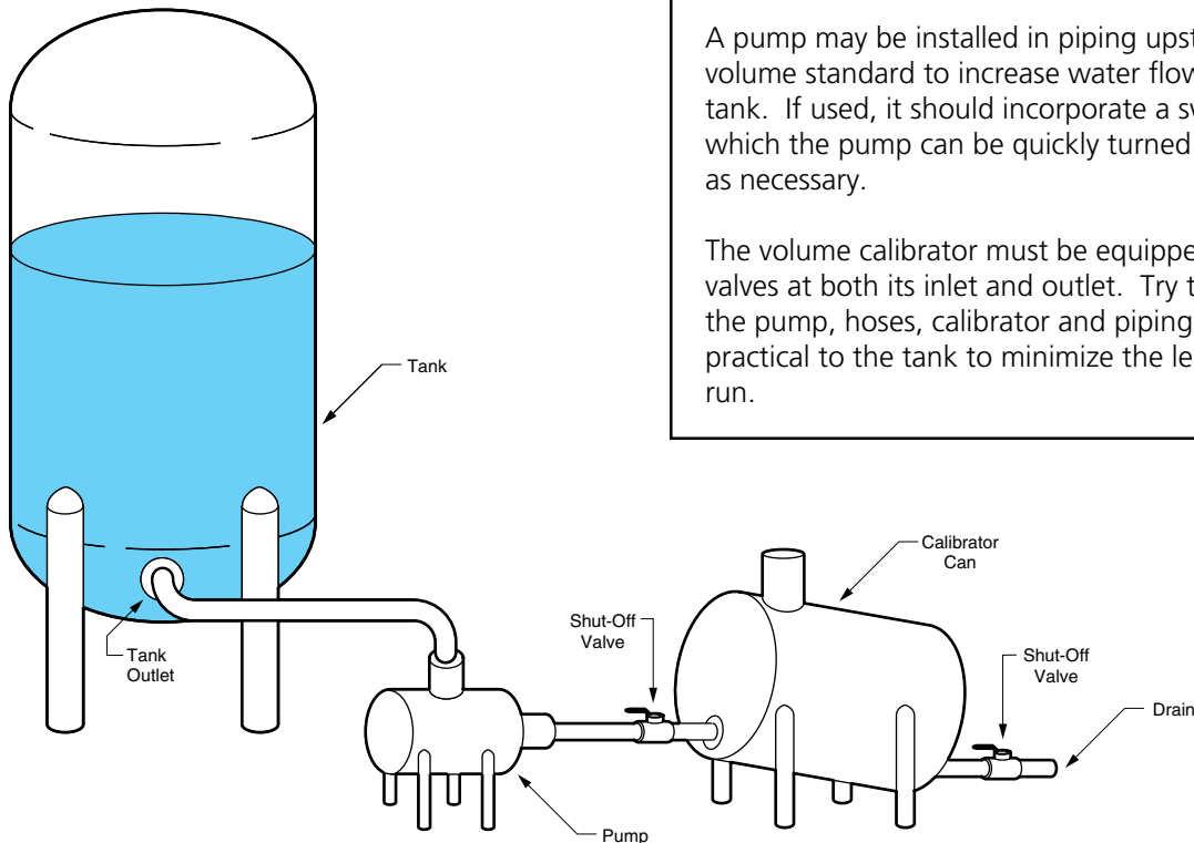
Recommended "Out" Calibration Procedure Using Volume Standard (Calibration)
