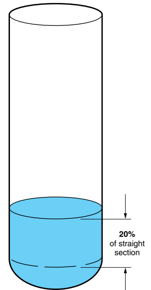
Minimum requirement for tanks greater than 15 ft.
