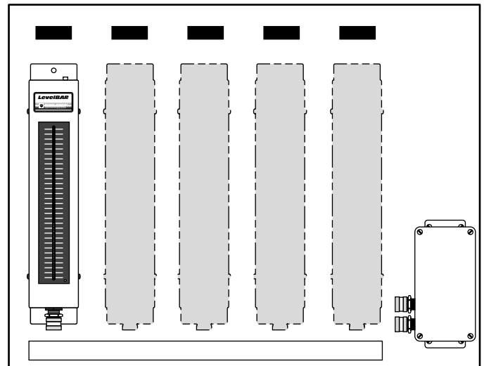
LevelBAR Column Indicator Panel
