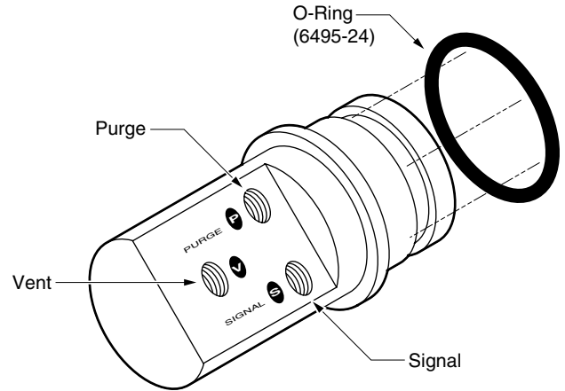
Detail 1 - Connector
