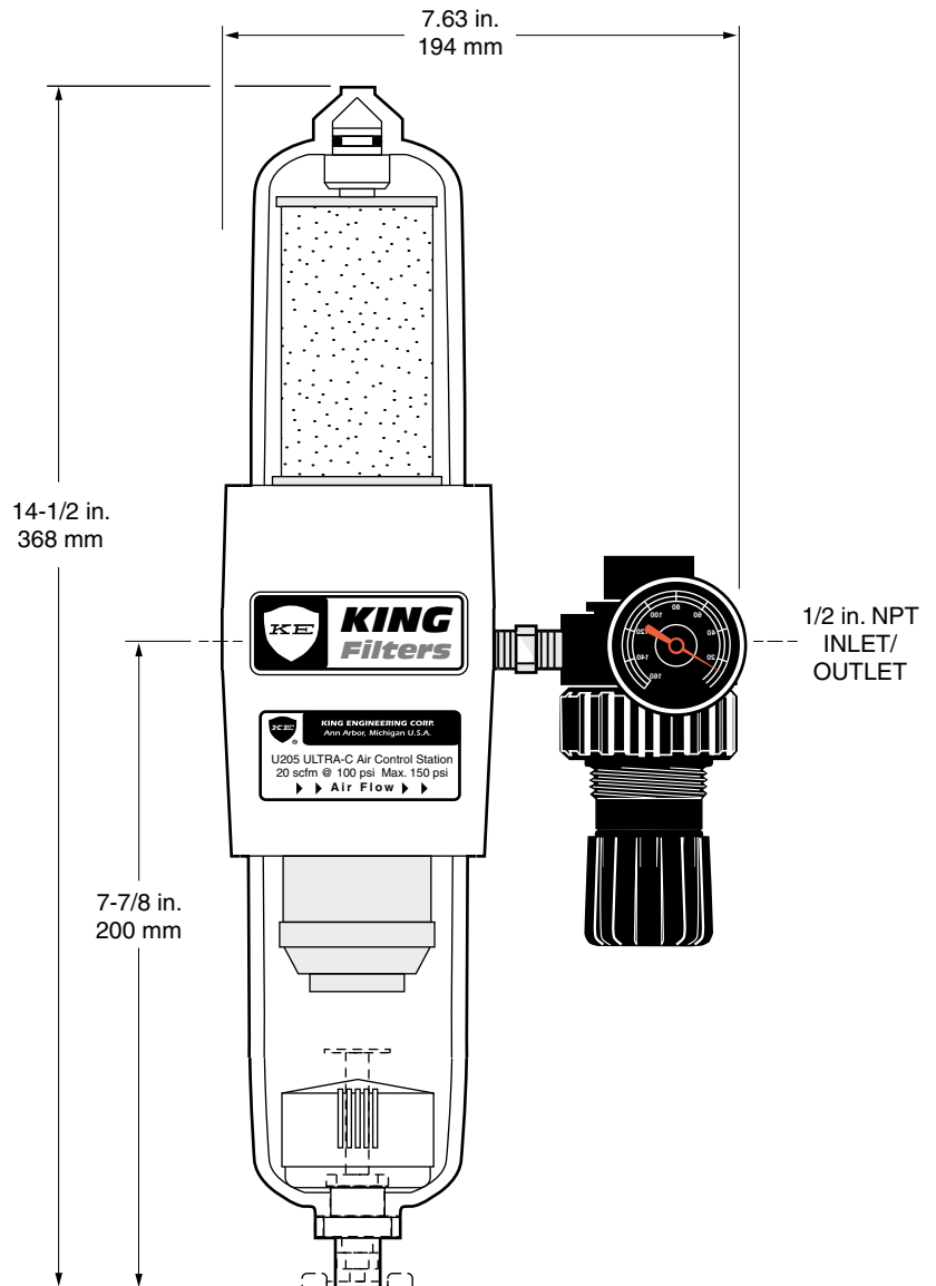
U205/U206 Two Stage Compressed Air Filter and regulator-gauge
