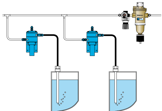
Air Control Station Model 72
