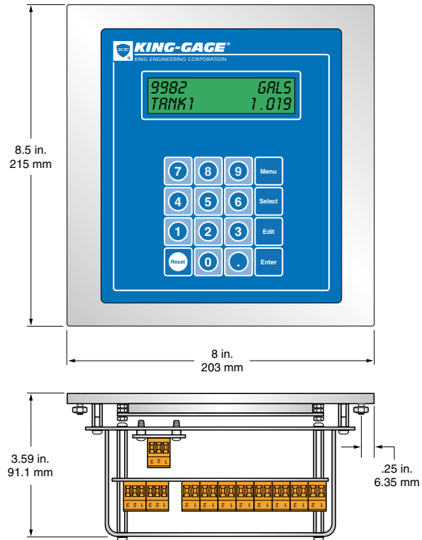
Model 4641-4-0
