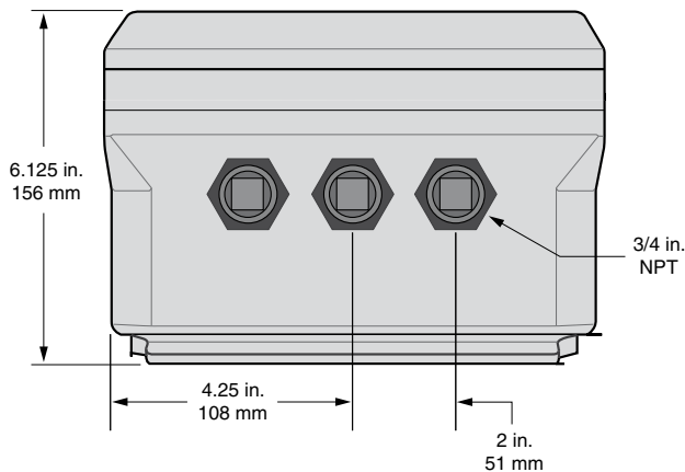
Model 4641-2-0
