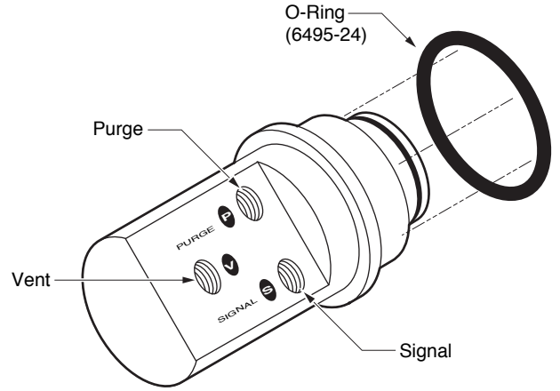
Detail 1 - Connector
