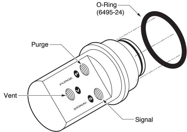
Detail 1 - Connector
