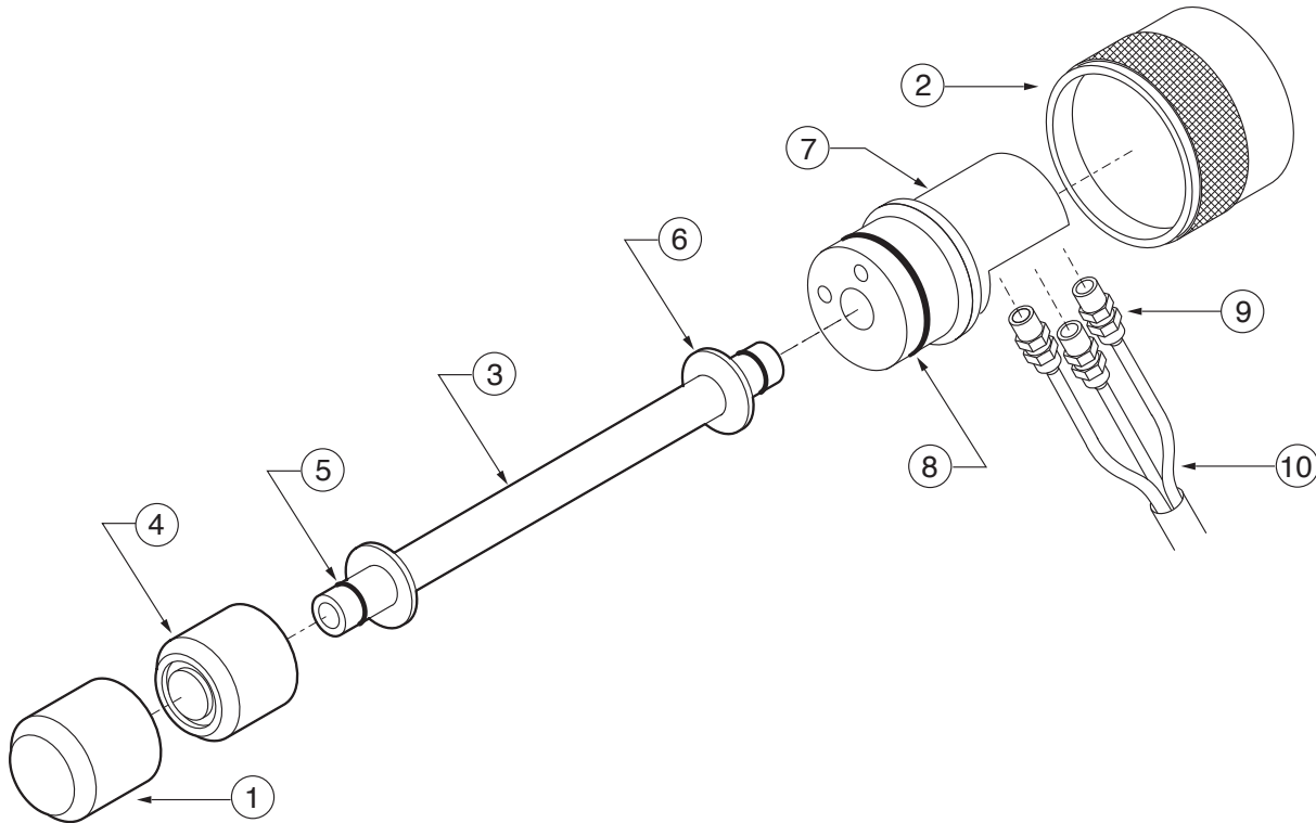
Figure 2 - Exploded view of typical sensor
