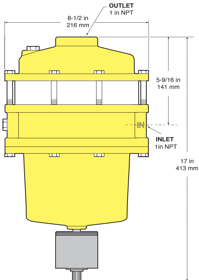
Filter w/ Automatic Drain
