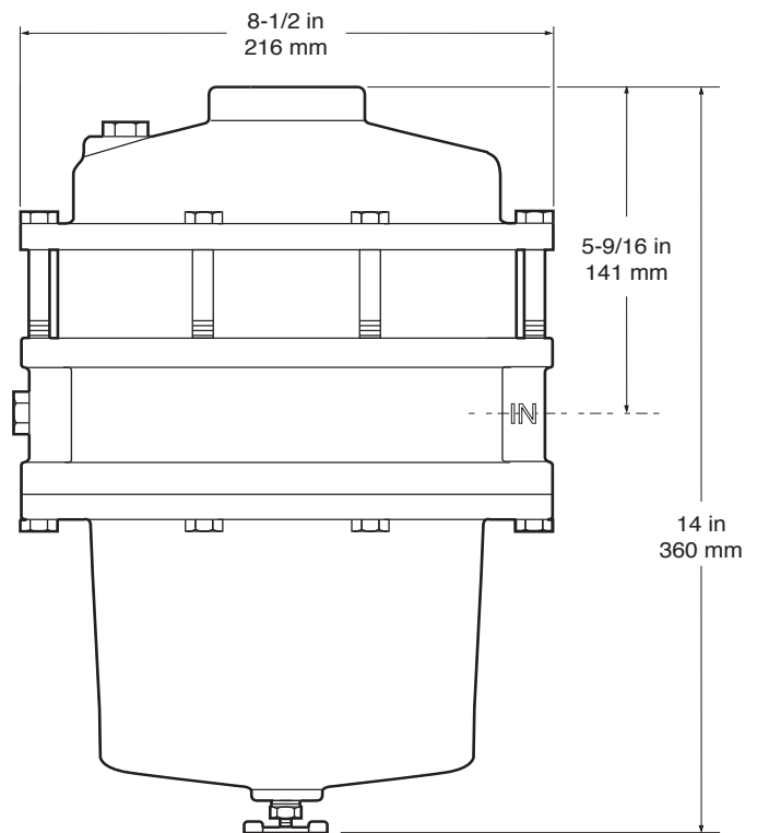
Filter w/ Manual Drain
